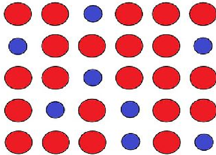
Substitutional alloy
